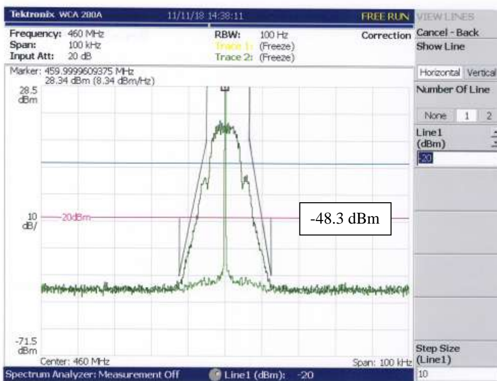
Fig. 1 Aclara Model 2011-009 Emissions Mask
