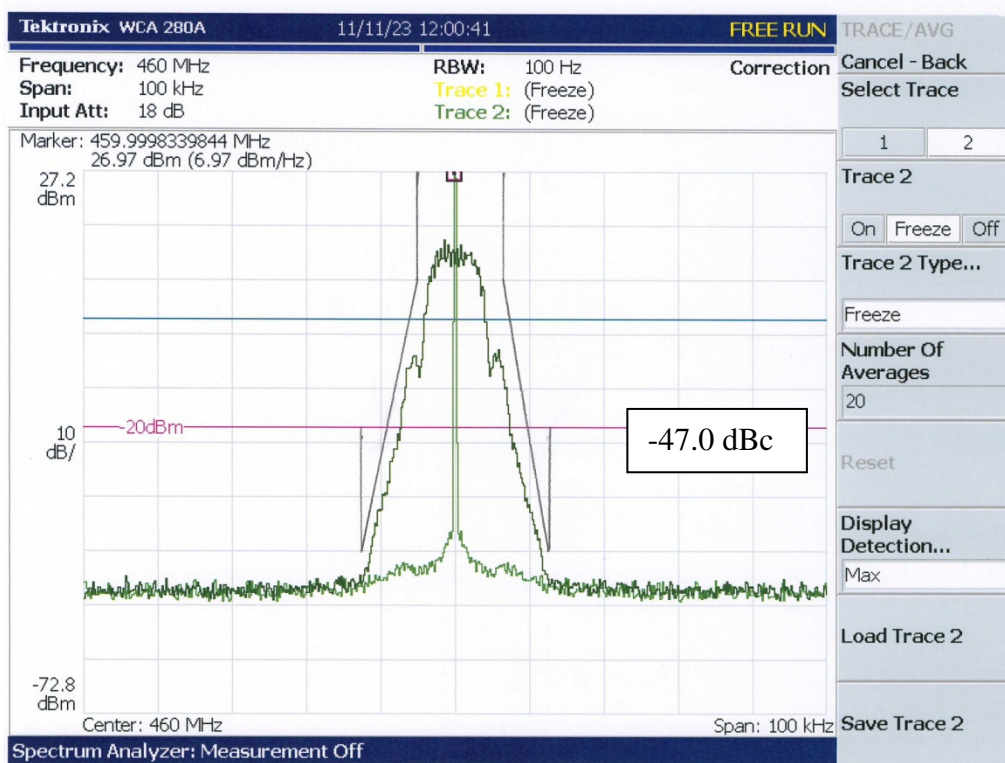
Fig. 1 Hexagram Model 2011-006X Emissions Mask
