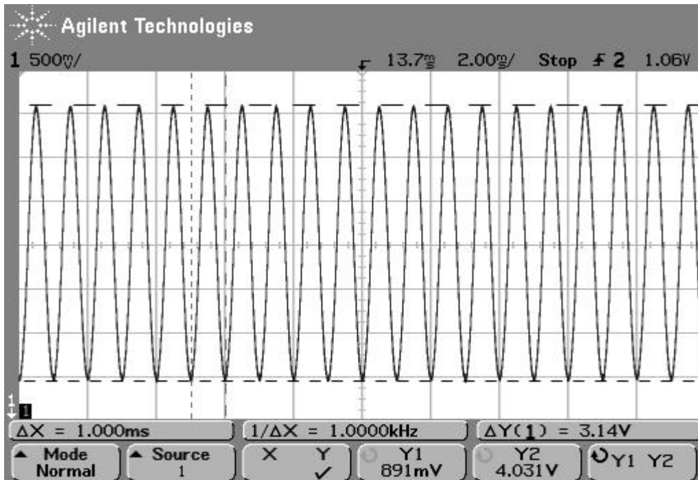
Fig. 3 \pm 12.5 kHz modulated test signal 25 kHz = 3.14 V.
