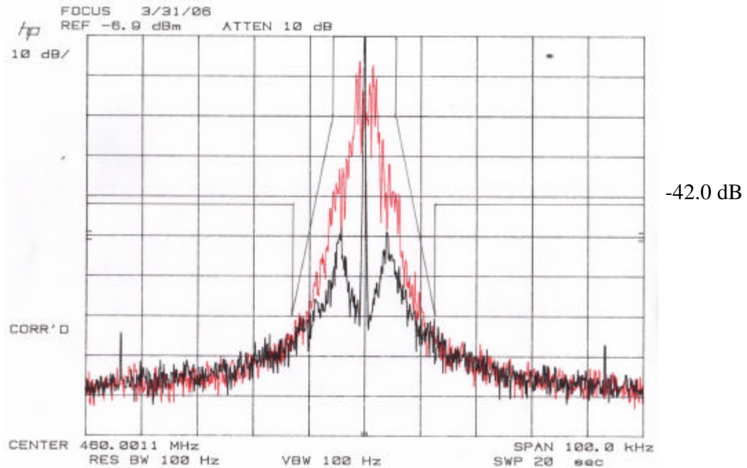
Fig. 1 Hexagram Model 10152 MTU Emissions Mask
