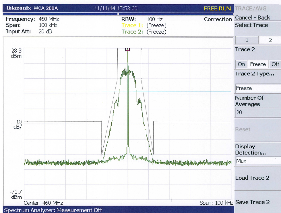
Fig. 1 Hexagram Model 2010-004X Emissions Mask
