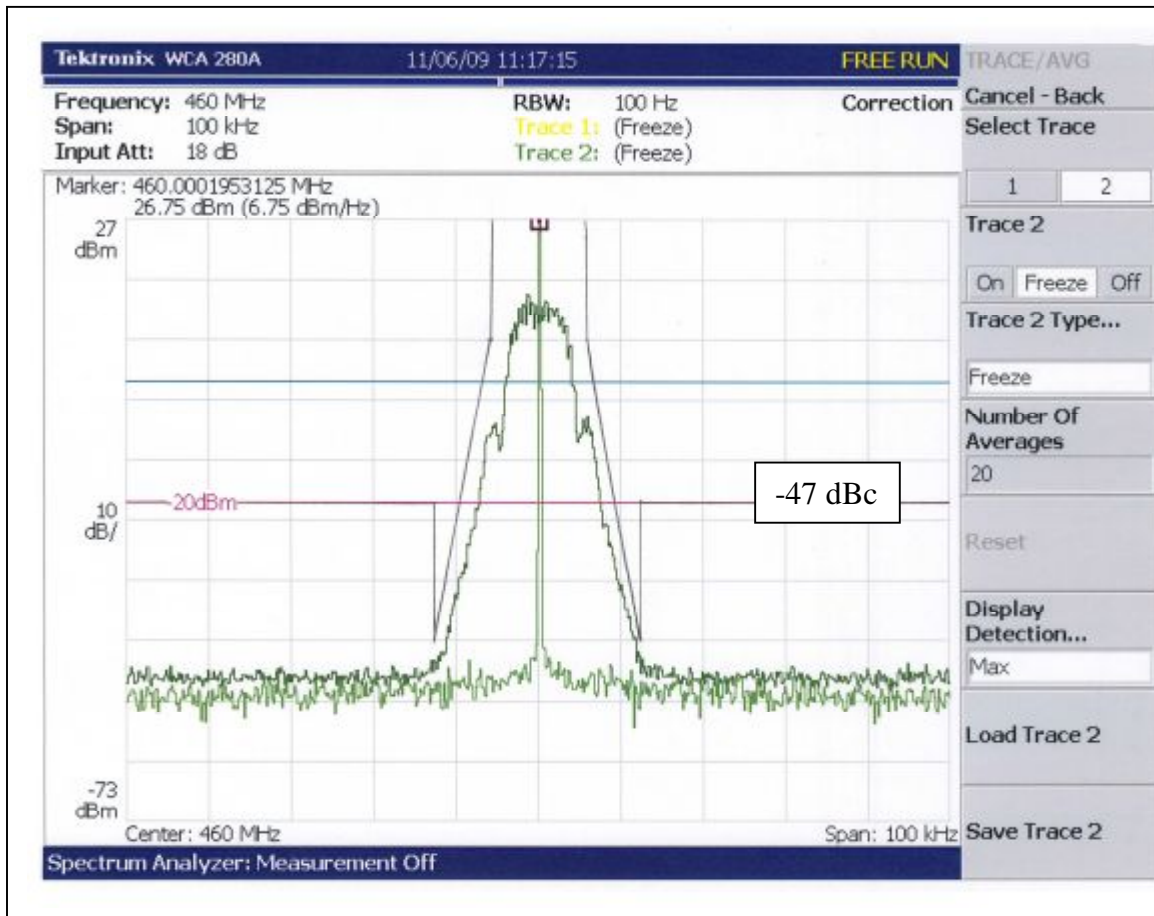
Fig. 1 Hexagram Model 2009-002G Emissions Mask
