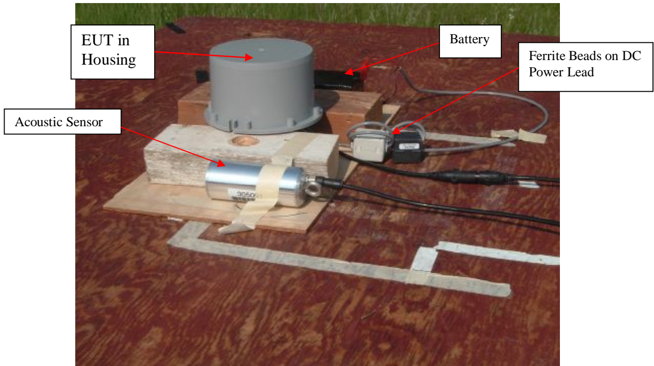
PICTORIAL 1 HEXAGRAM MODEL 2009-002G MTU OUTPUT POWER AND SPURIOUS EMISSIONS TYPICAL TEST SETUP
