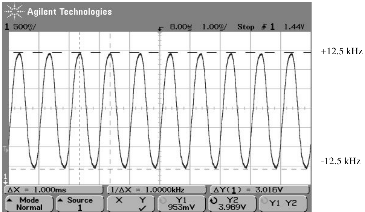
Fig. 3 ±12.5 kHz modulated test signal .
