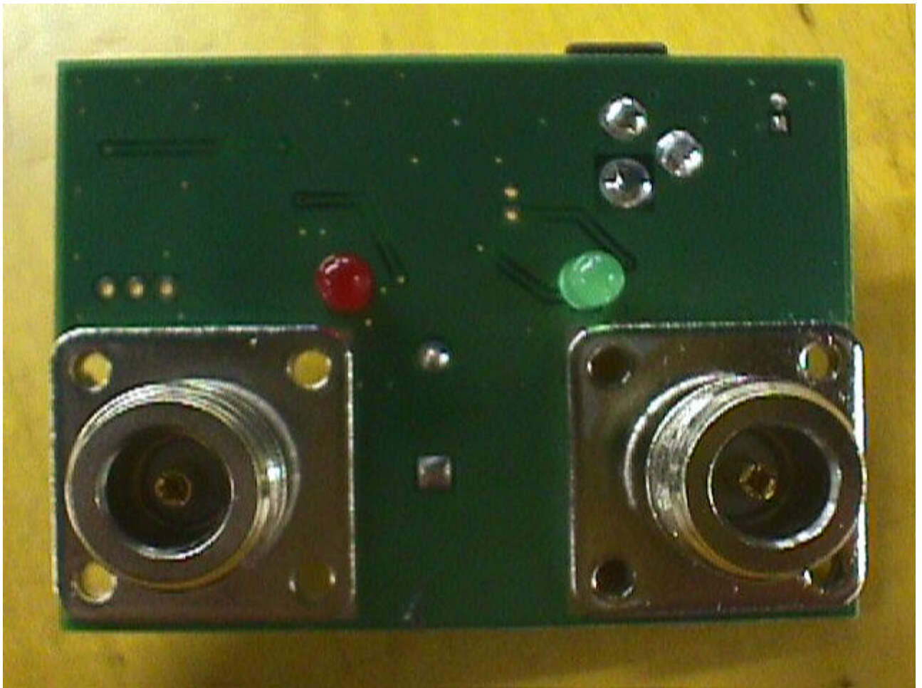
G9: DC POWER INJECTOR SOLDER SIDE VIEW
