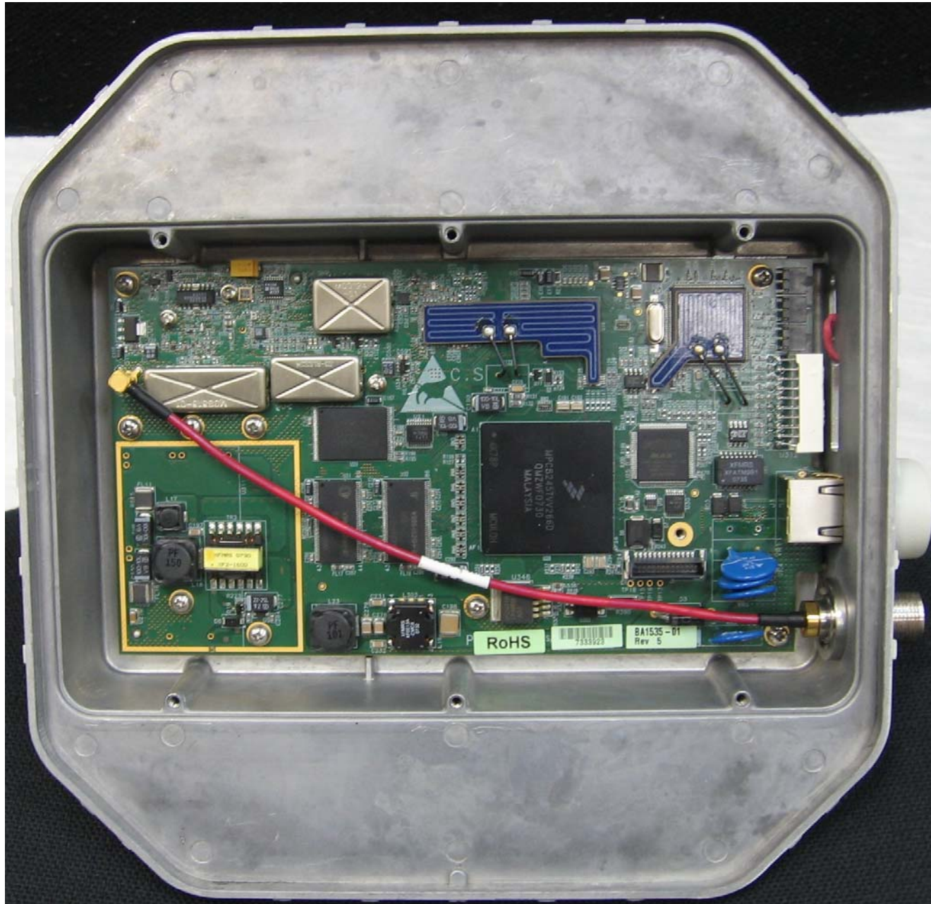
Photo5. Unit inside enclosure view
