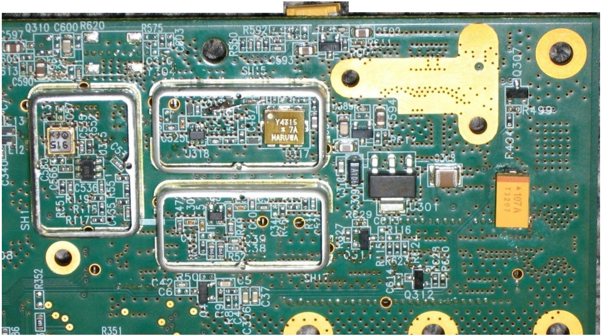
Photo9. RF block details
