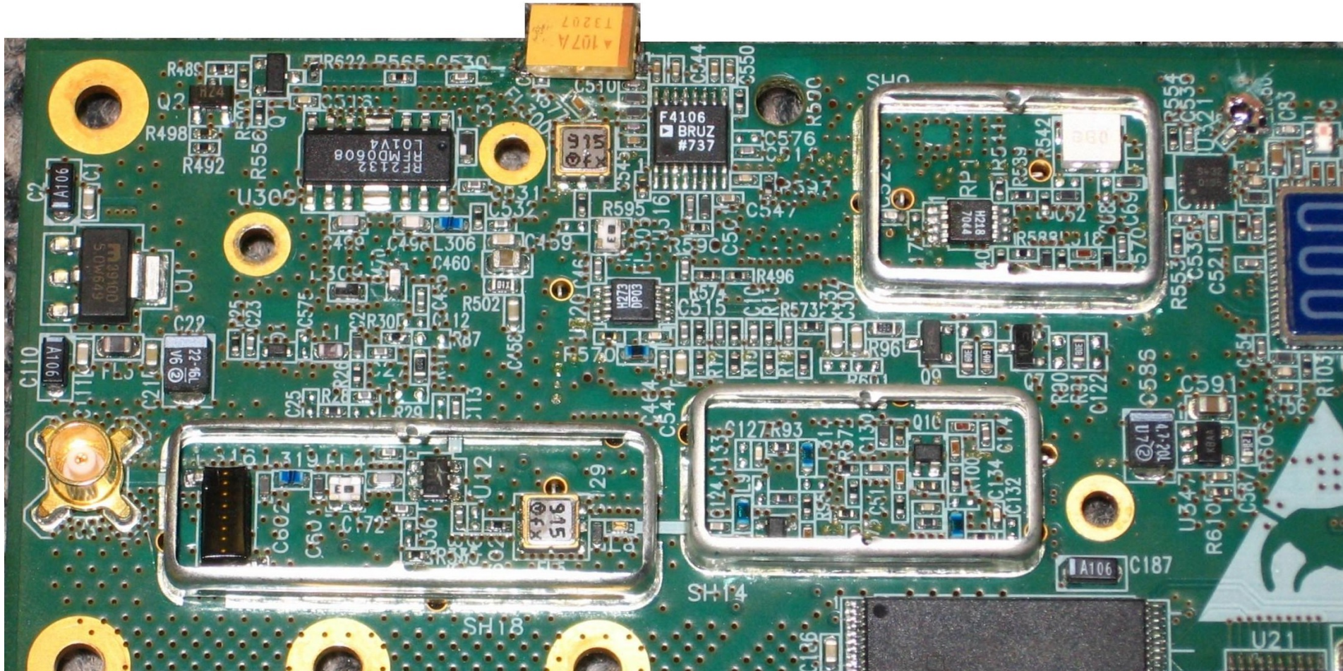
Photo8. RF block details
