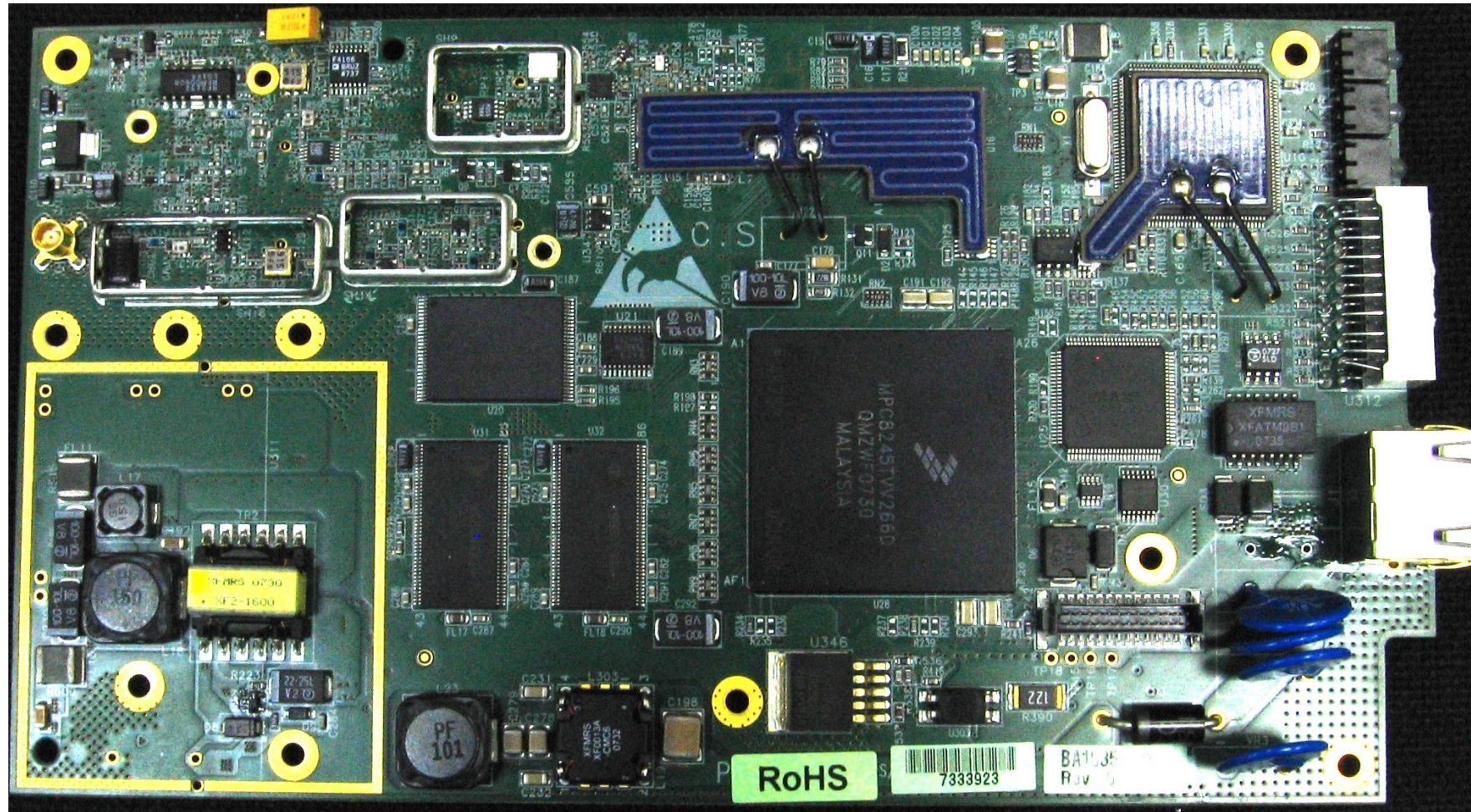
Photo6 . PCB components side
