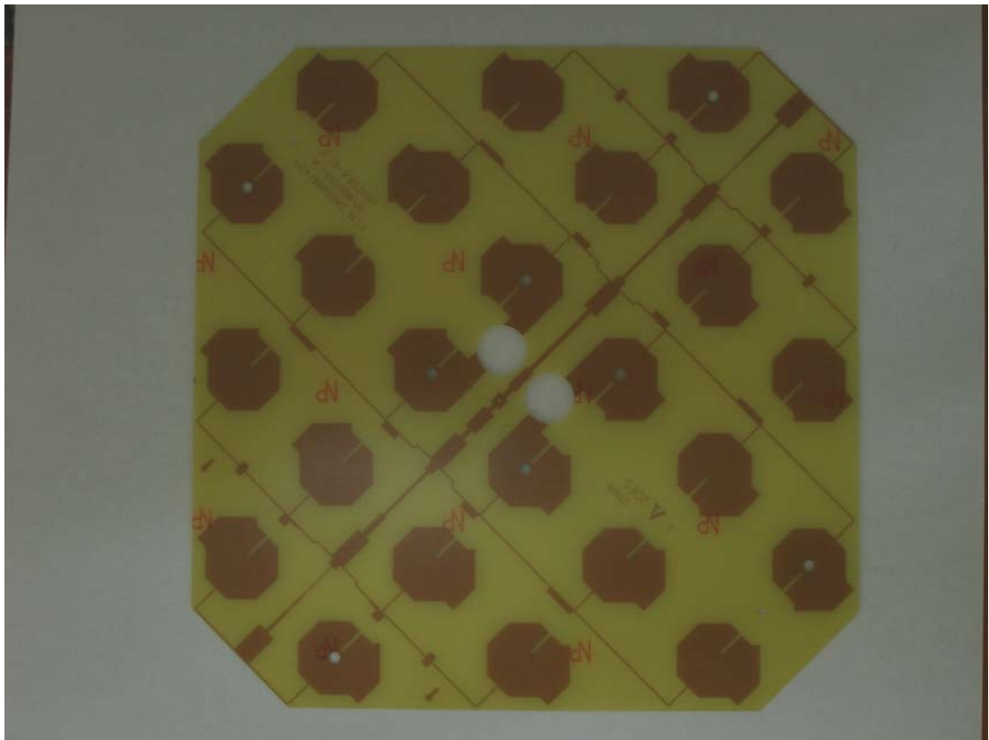
ODU antenna , opposite to print side
