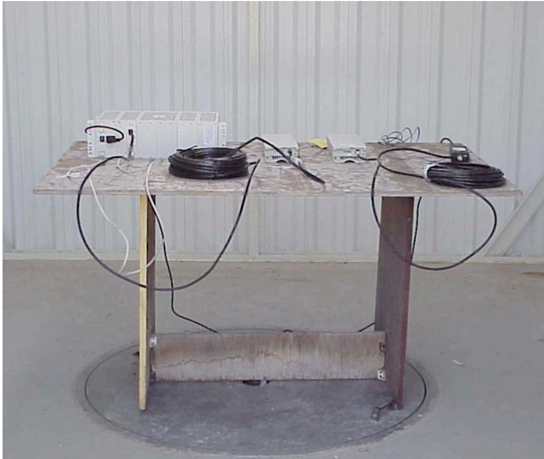
Photo# 2. Radiated emission open site test
