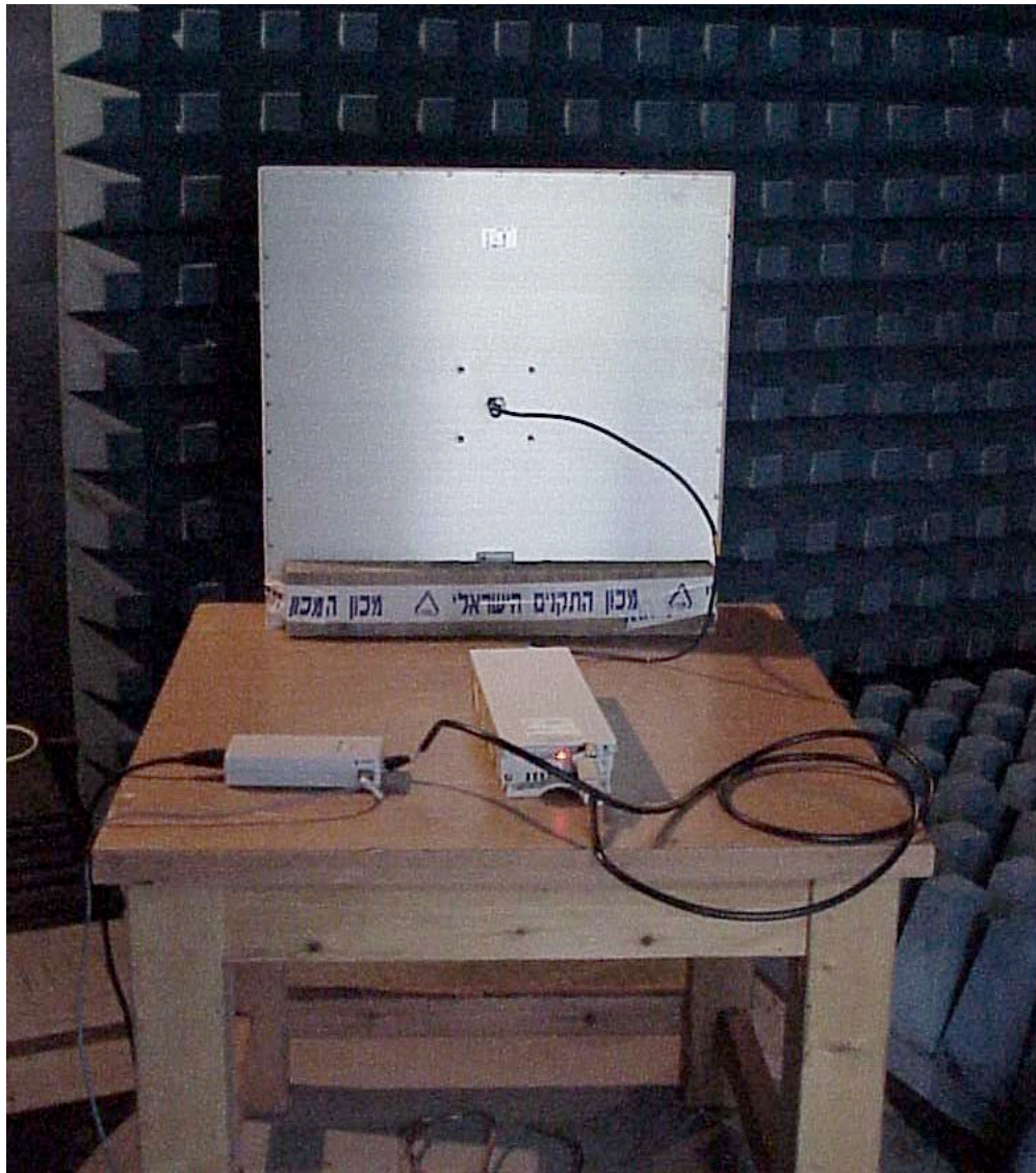
Photo# 7. Radiated spurious emission test . Antenna P/N AN1230
