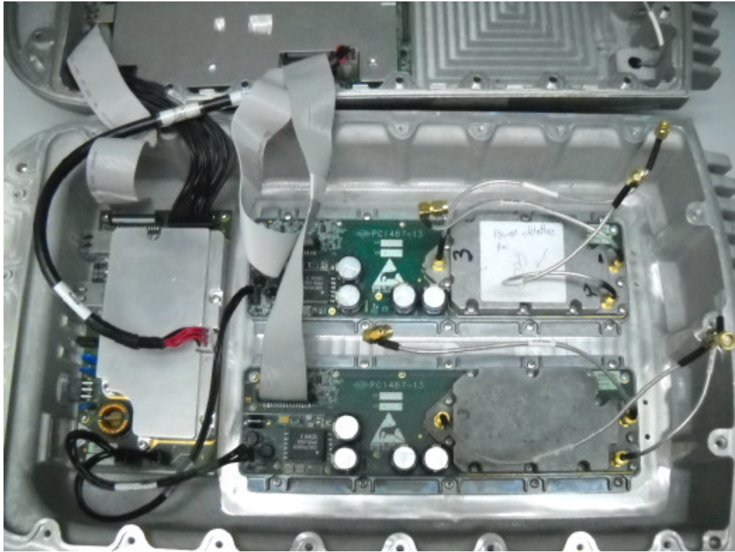
Photograph No.1 BreezeMAX Micro Outdoor microbase station internal view
