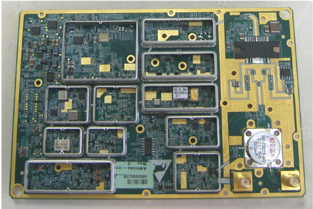
Photograph No.5 Radio module printed circuit board front view with shields removed
