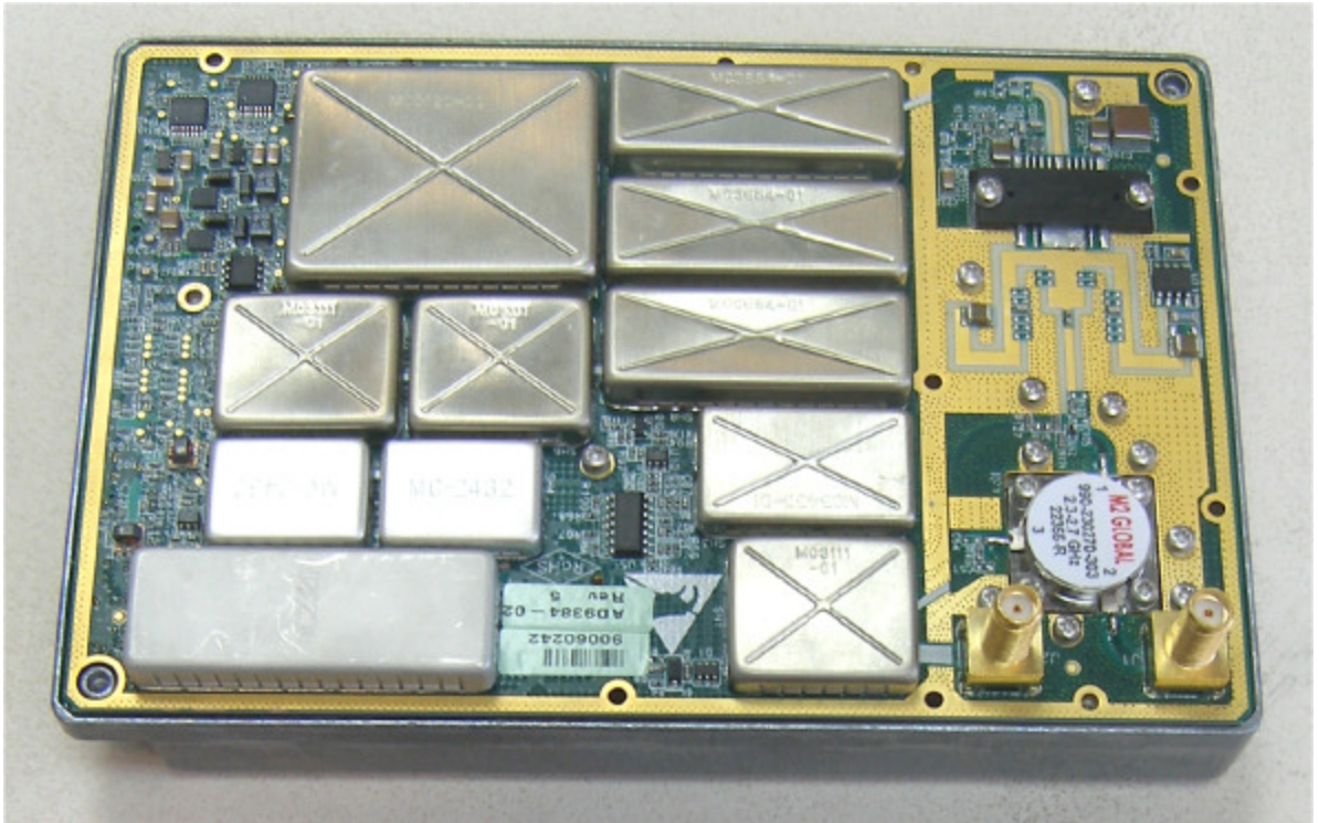
Photograph No.4 Radio module printed circuit board front view
