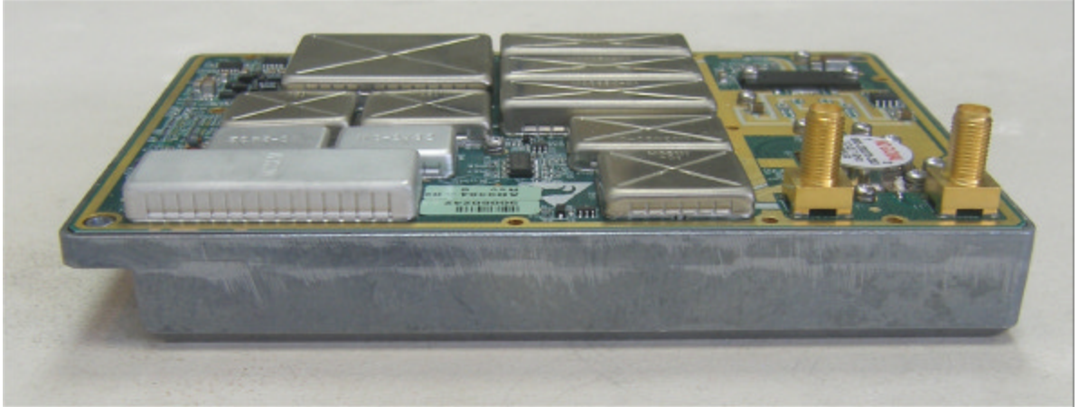
Photograph No.3 Radio module view without cover
