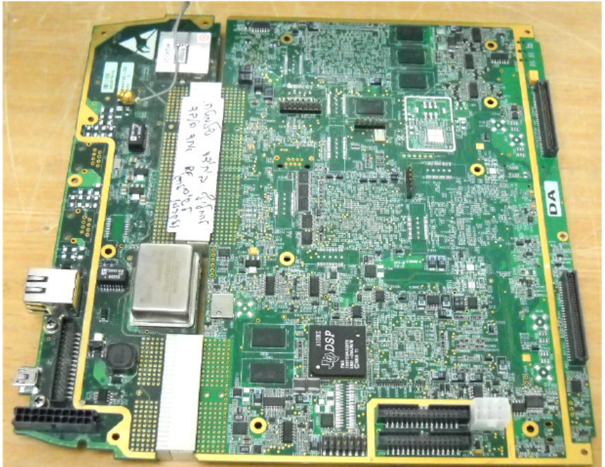
Photograph No.10 Digital PCB front view
