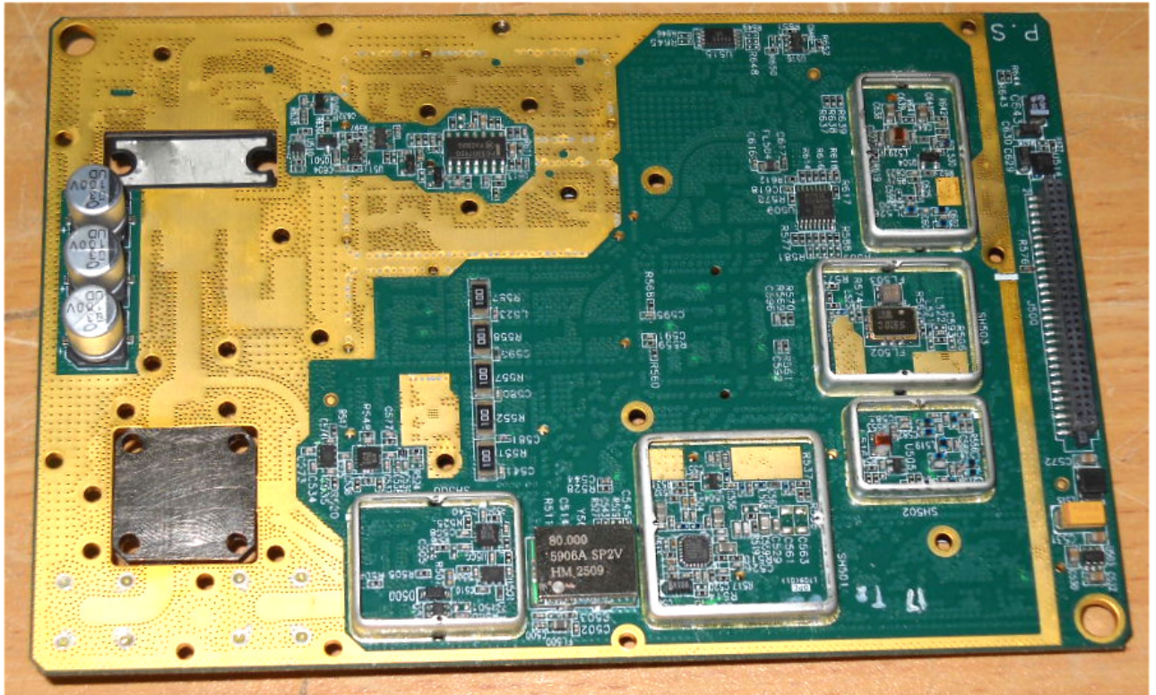
Photograph No.7 RF module second side without shields
