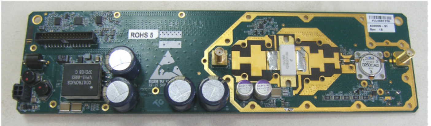
Photograph No.8 High Power Amplifier PCB front view
