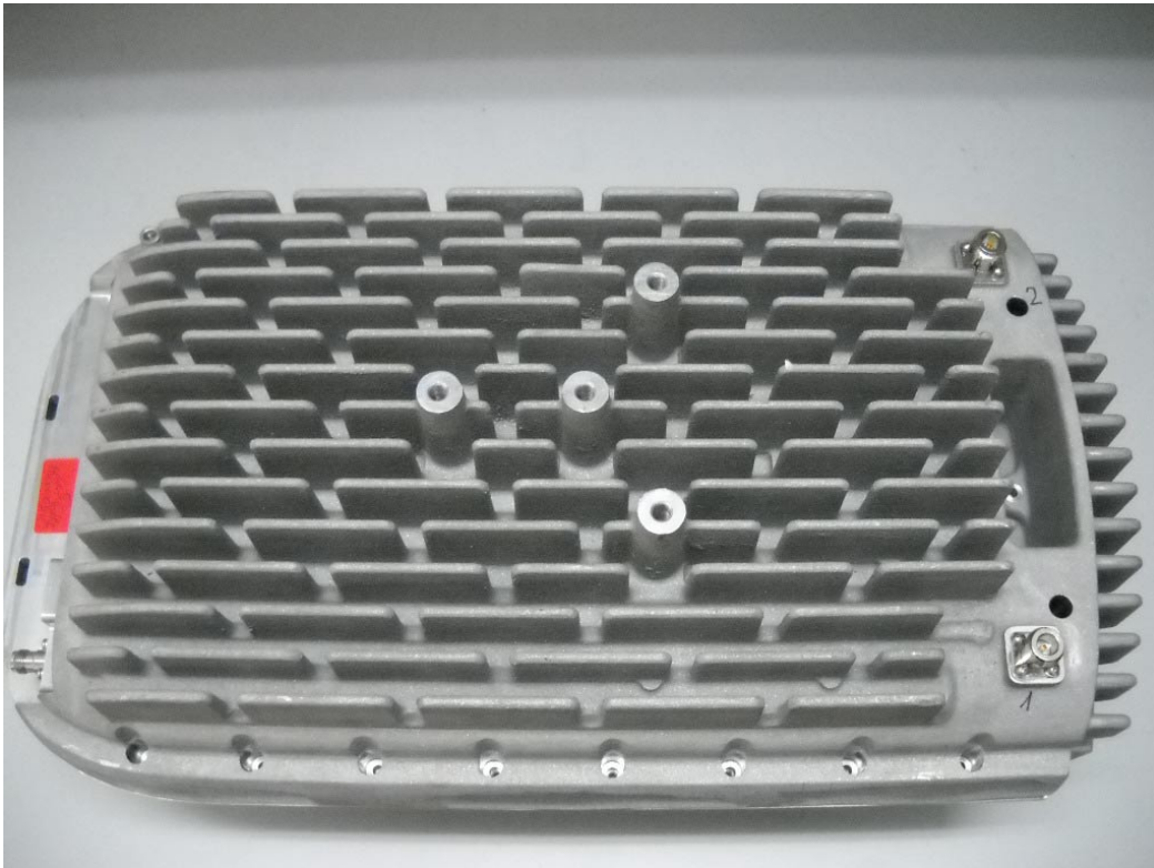
Photograph No.1 BreezeMAX Micro Outdoor microbase station front view
