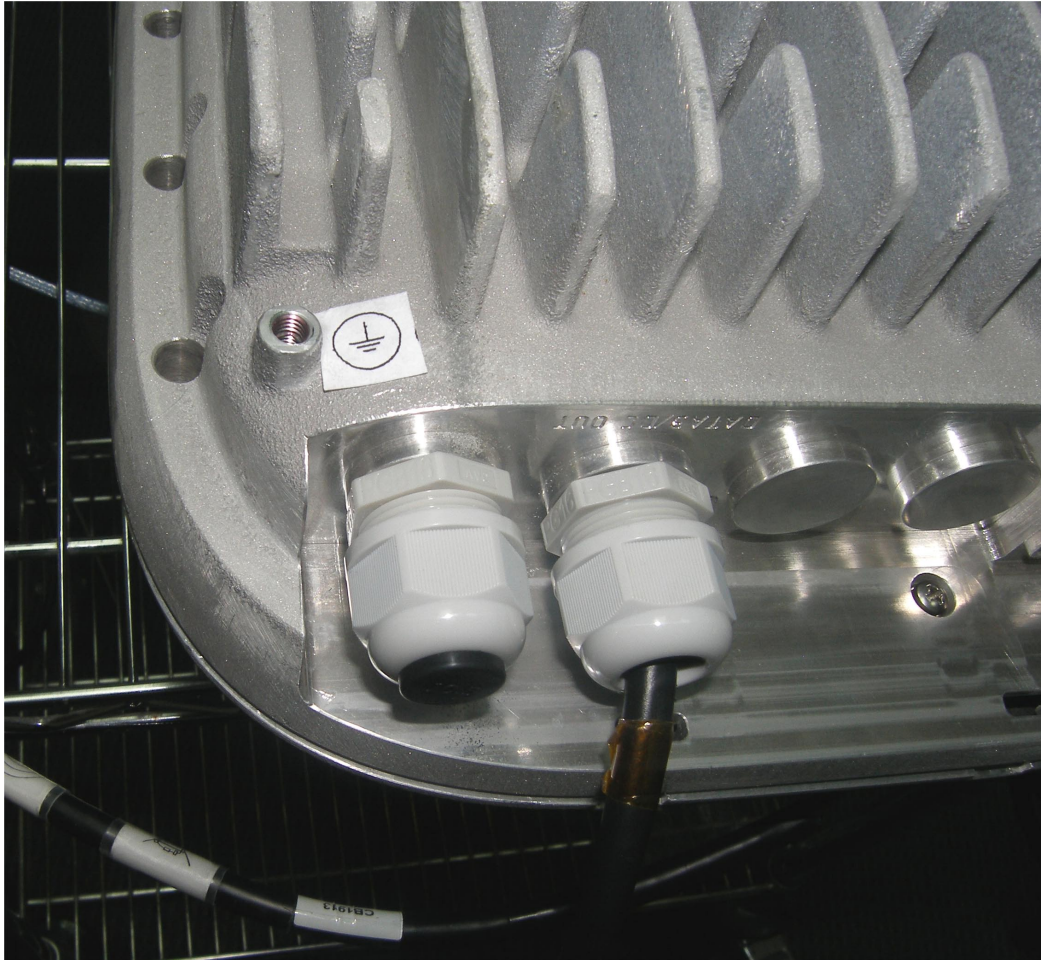
Photograph No.4 BreezeMAX microbase station connectors general view
