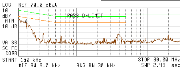
Plot 4. Conducted emissions measurement result on CX-BA2.4-BA900 Reference standard: FCC Part 15 class B Test line: Neutral
