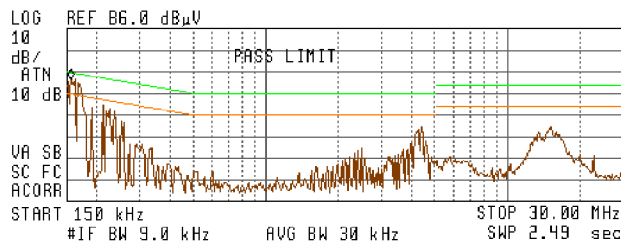
Plot 2. Conducted emissions measurement result on CX-VL5.8-BA900
