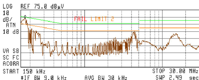
Plot 1. Conducted emissions measurement result on CX-VL5.8-BA900
