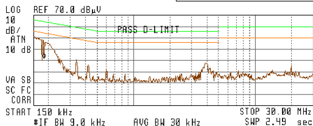
Plot 3. Conducted emissions measurement result on CX-BA2.4-BA900 Reference standard: FCC Part 15 class B Test line: Phase
