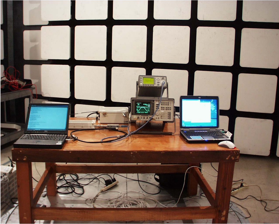
Antenna conducted emissions setup
