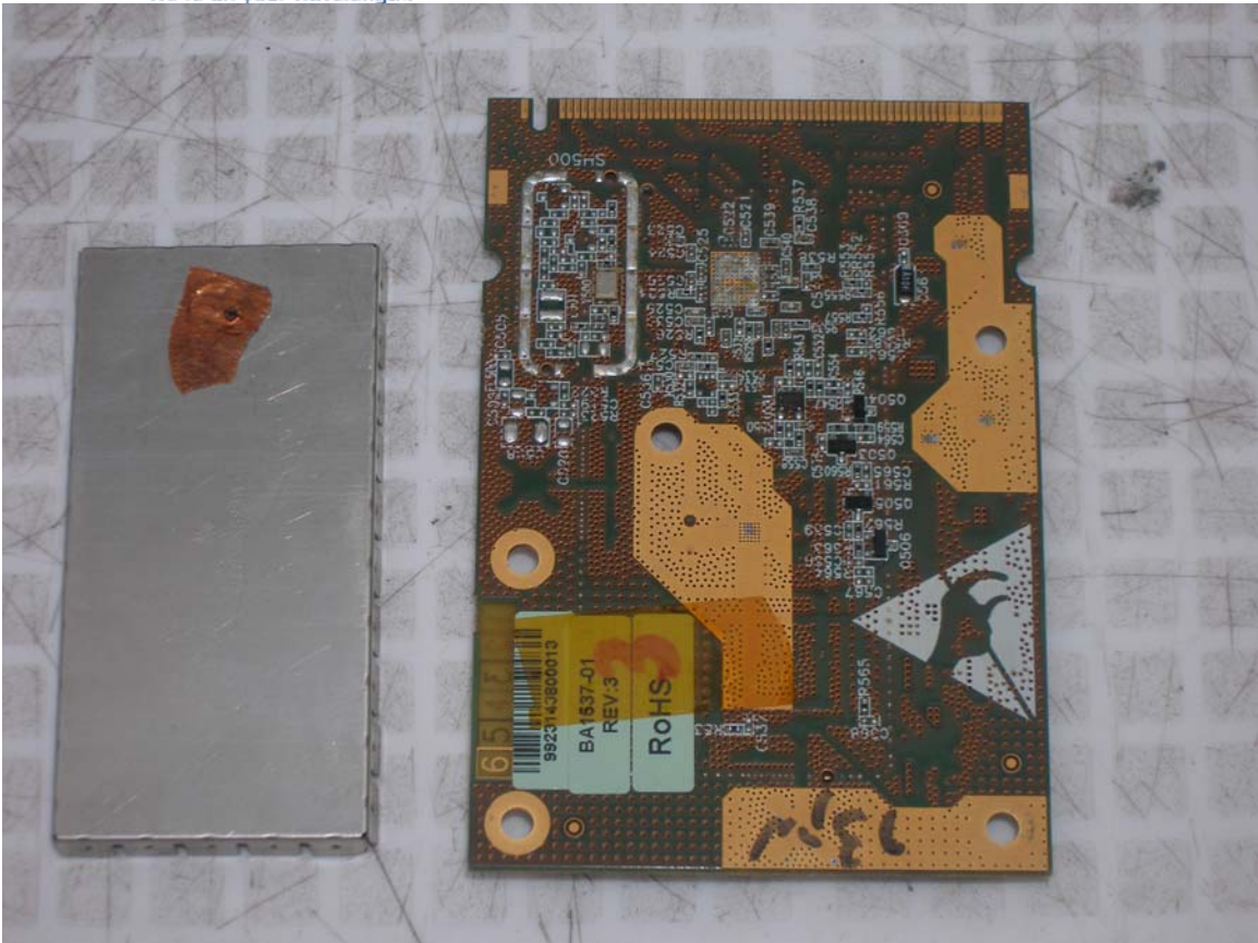
Photo8. Radio module, PS view.
