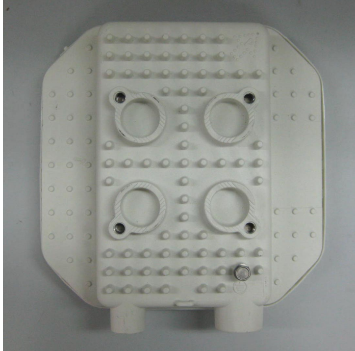
Photograph No.3 BreezeMAX Extreme 5GHz CPE rear side view
