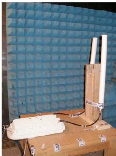
Photo #4. Test setup with external Omni antennas.
