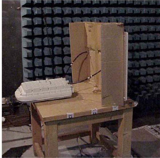
Photo #5. Test setup with external sector antennas.
