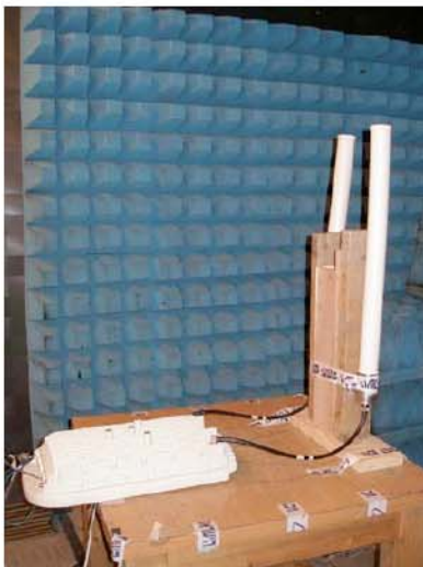
Photo #4. Test setup with external Omni antennas.
