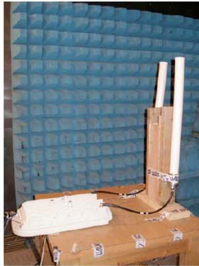
Photo 4. Investigation test setup with external Omni antenna.
