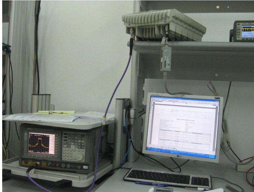
Photograph No.2 Emission mask, conducted spurious emissions and occupied bandwidth measurement setup
