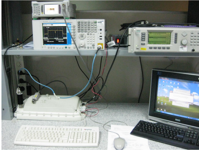
Photograph No.2 Occupied bandwidth, emission mask measurement setup
