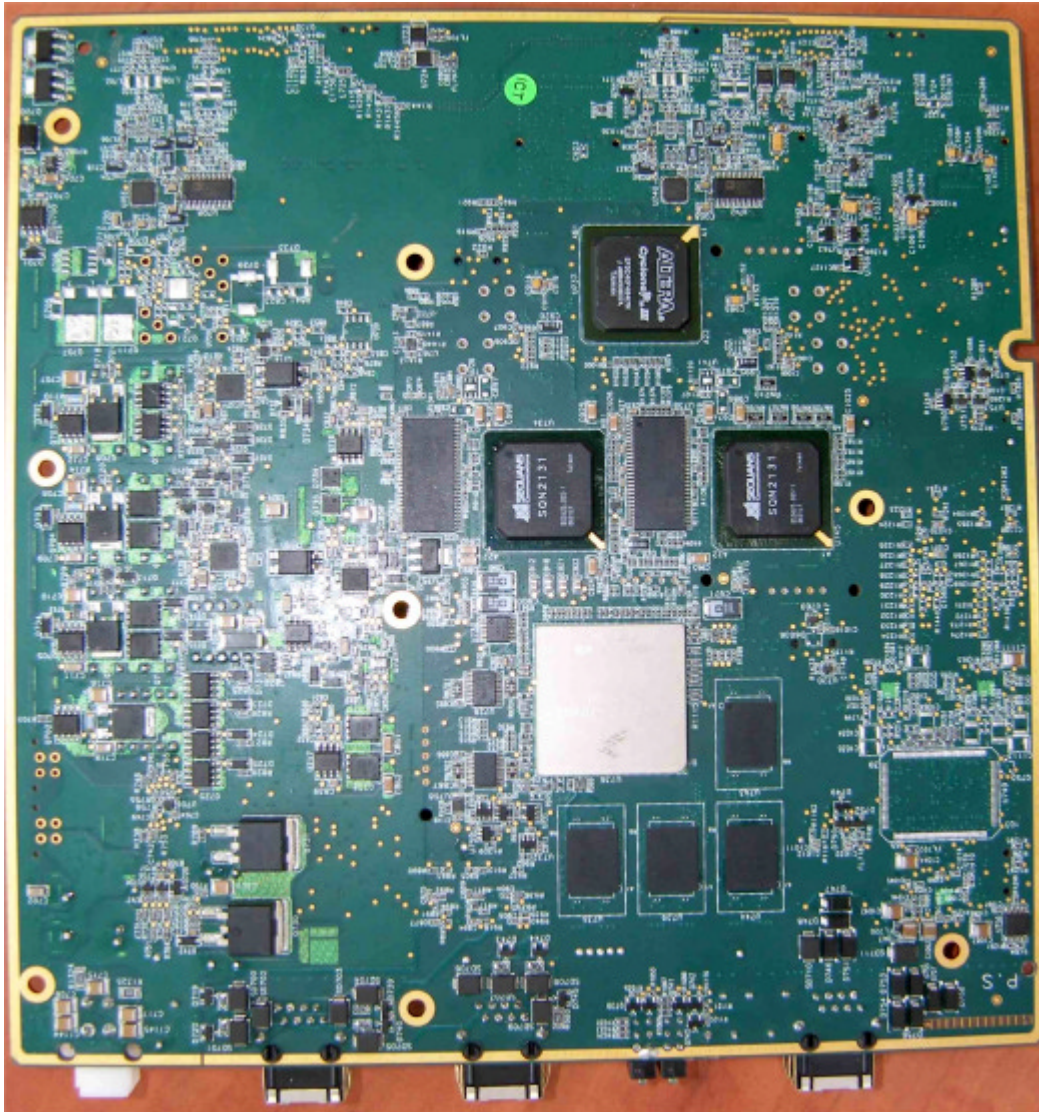
Photograph No.10 Digital PCB second side view
