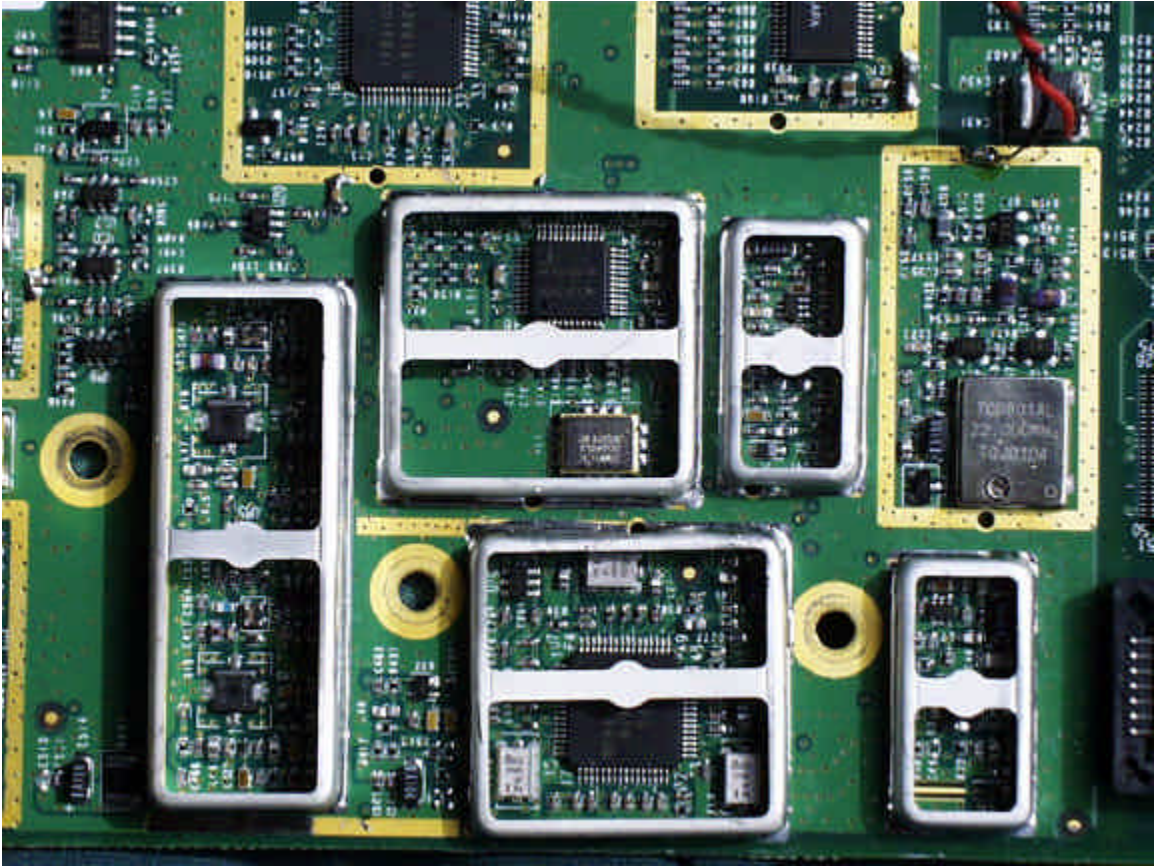
Outdoor radio unit, radio board component side with cans removed
