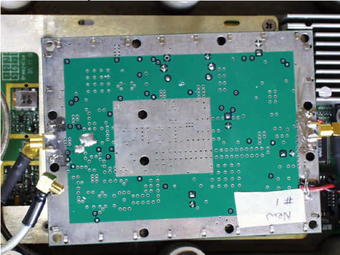
Outdoor radio unit, up/down converter unit, board bottom
