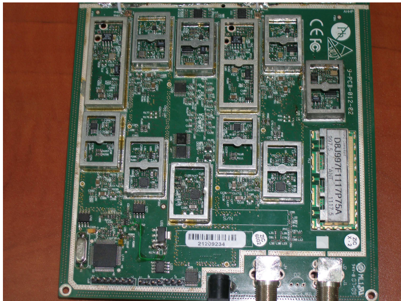
With shielding case removed
