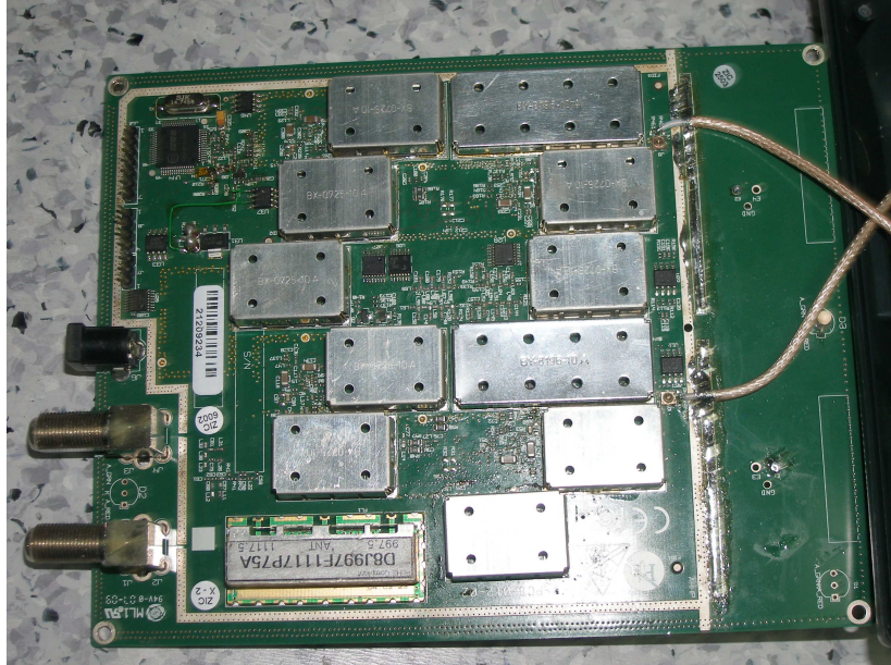
Photograph No.3 Component side view
