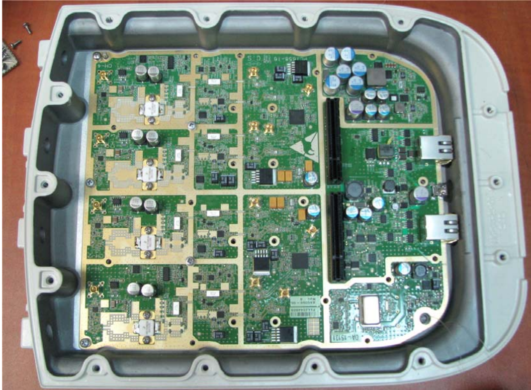
Photograph No.3 Base station RF part top internal view
