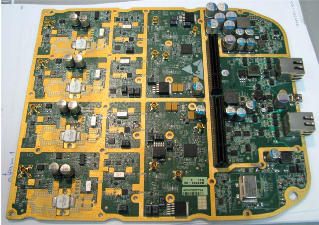
Photograph No.4 RF part PCB top view
