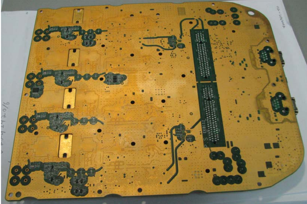
Photograph No.5 RF part PCB second side view
