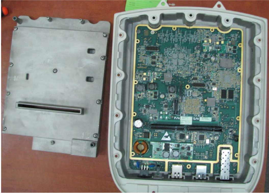
Photograph No.7 BreezeCOMPACT base station digital part with screen removed
