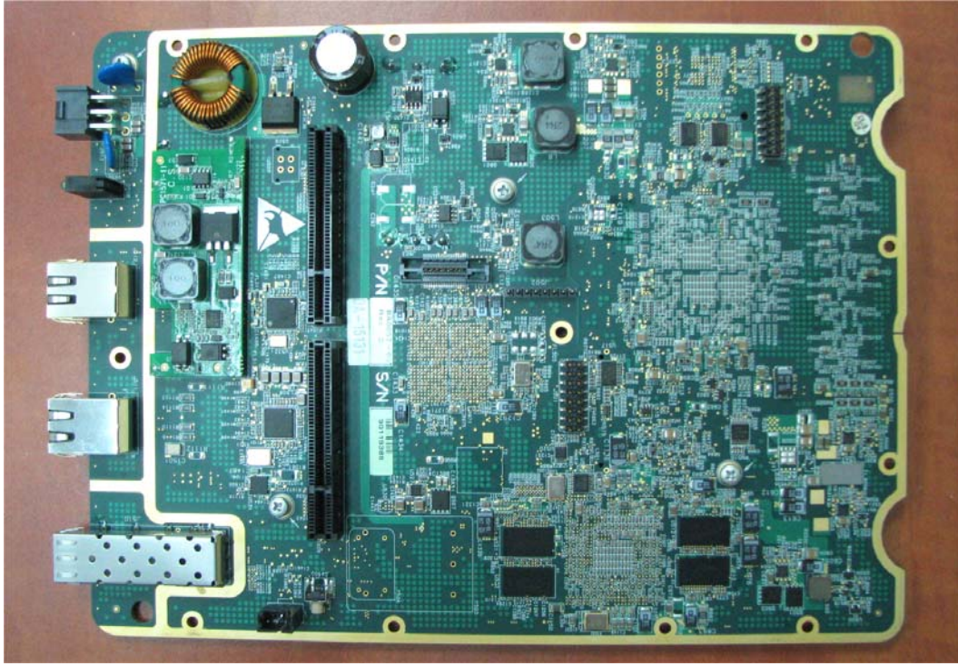
Photograph No.8 Digital part PCB top view
