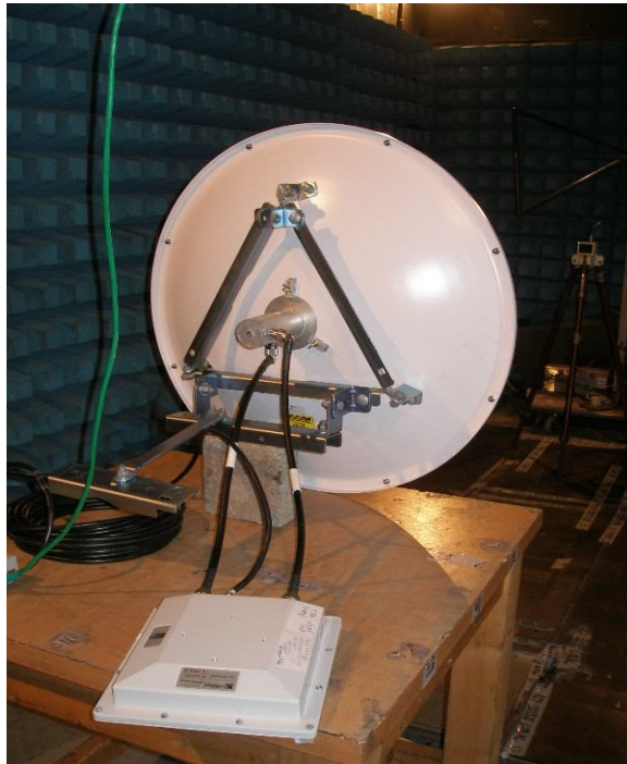
Photo 5. Radiated emissions test setup with parabolic antenna.
