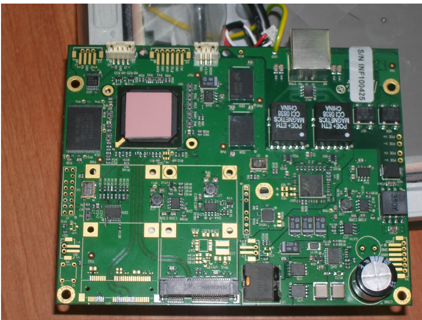
Photo 3. PCB PS without radio module
