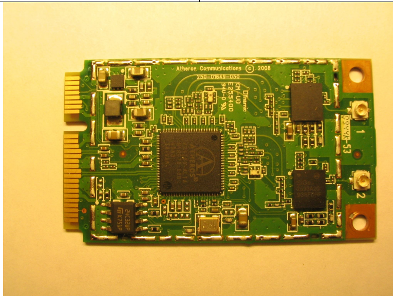
Photo 7. Radio module. Front view without shield.
