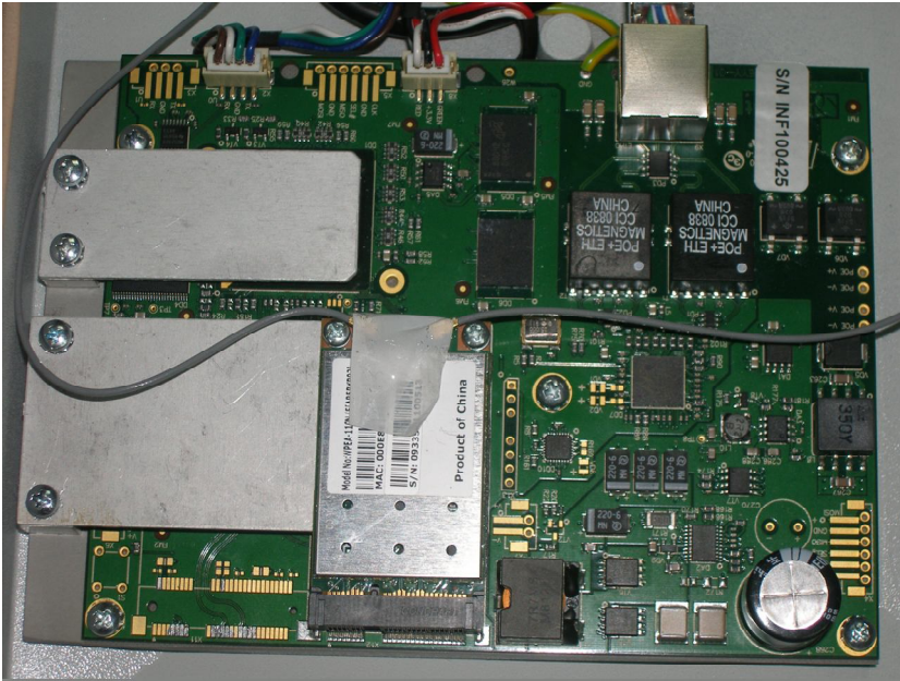
Photo 2. PCB PS with radio module
