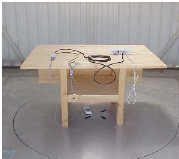
Photo #2. Radiated emissions test setup on OATS.
