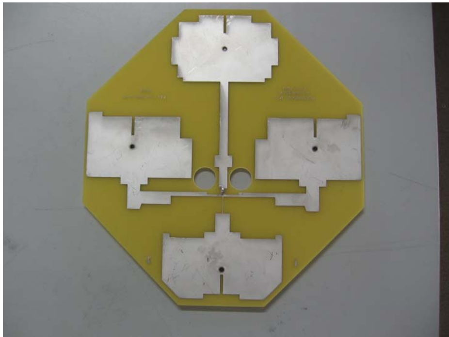
Integral Antenna Side 1
