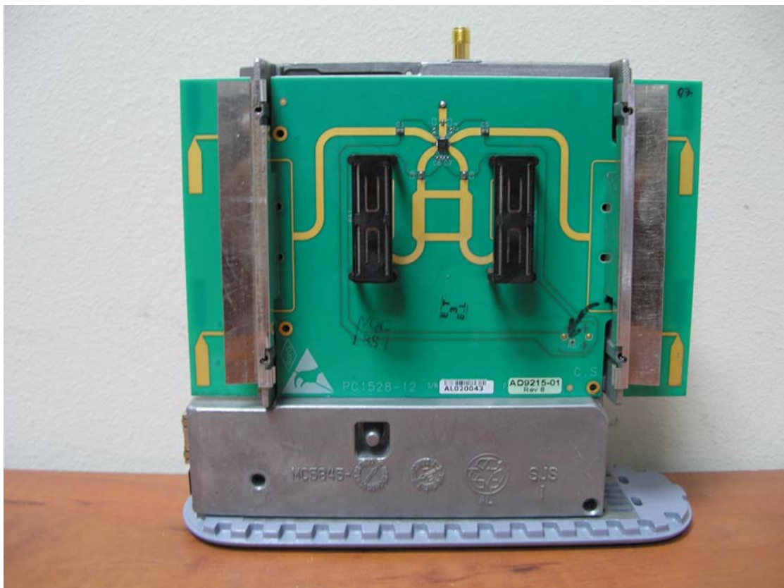
Photo7. Antenna
