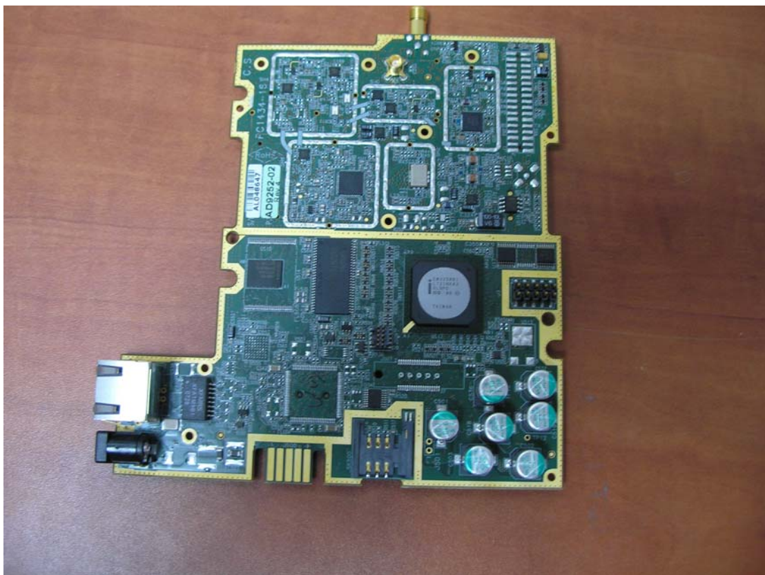
Photo3. PCB components view
