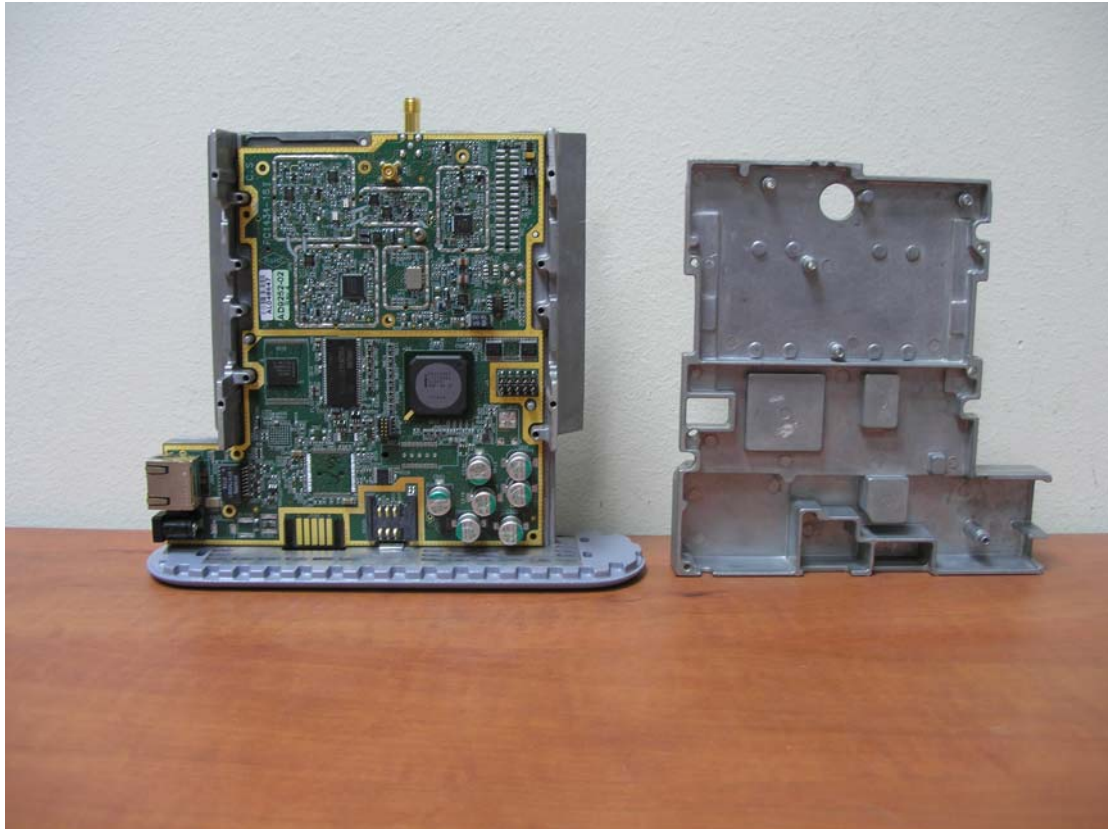
Photo2 . cover removed . components view.
