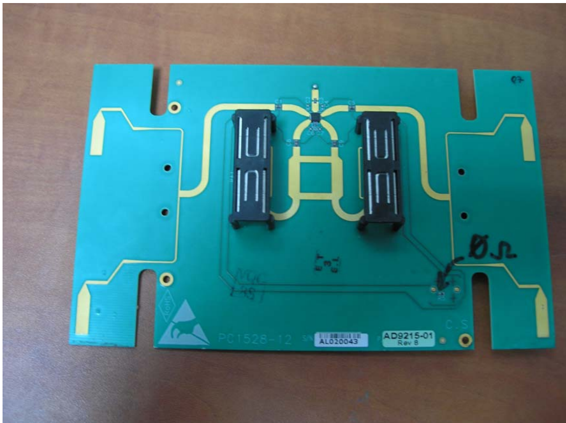
Photo 5. internal antenna
