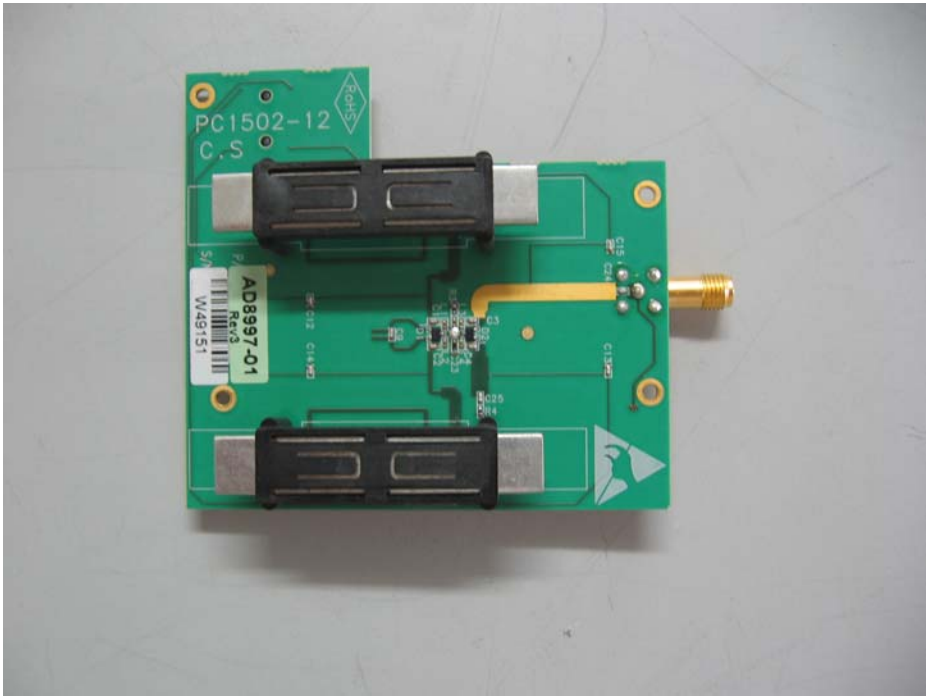
Internal Antenna 5,6 Component Side
