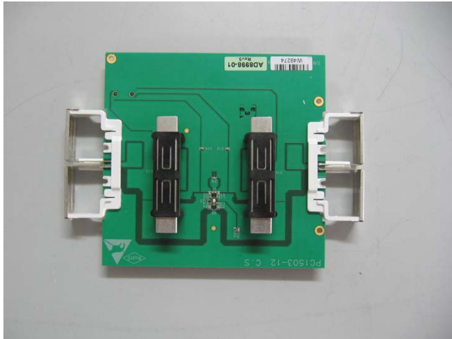
Internal antenna 1-4 Component Side
