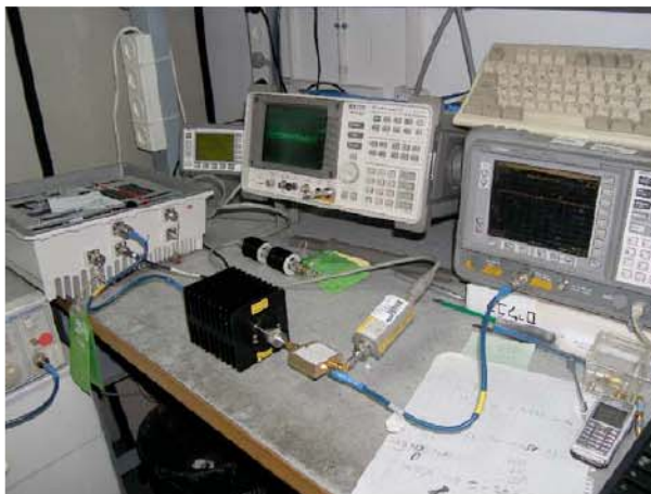
Photo 1. Conducted measurements. Test setup.
