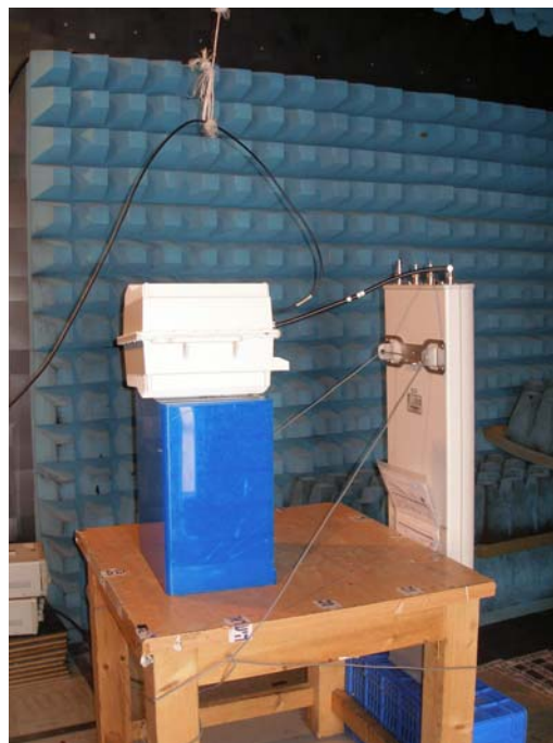
Photo 2. Test setup in anechoic chamber..
