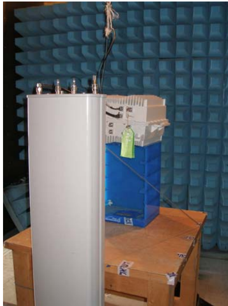
Photo 3. Test setup in anechoic chamber.
