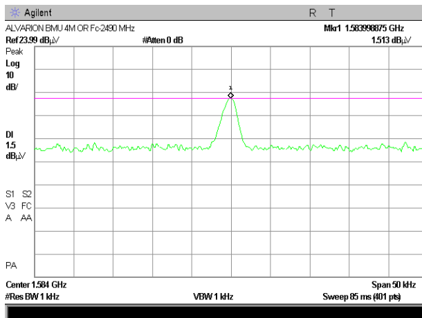
Plot # 15. Narrow band limit -80 dBm/kHz
