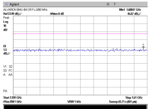
Plot # 16. Narrow band power density.
