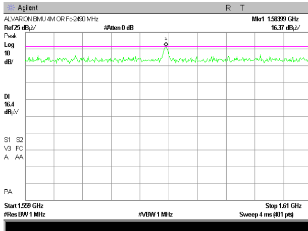
Plot # 13. Wide band limit -70 dBm/MHz.
