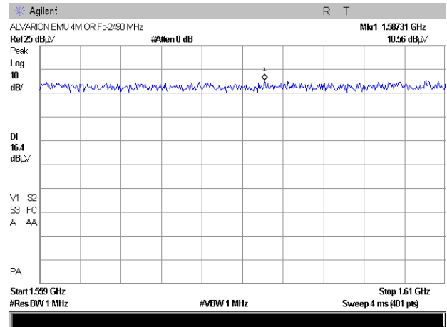
Plot # 14. Wide band power density
