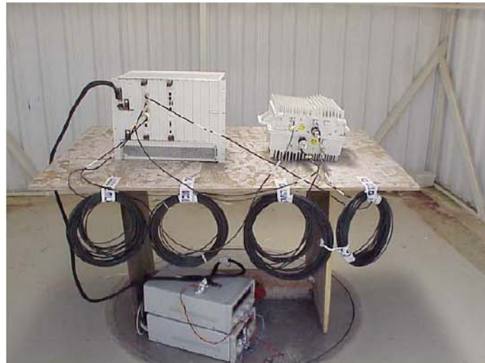
Photo 2. Test setup on OATS.
