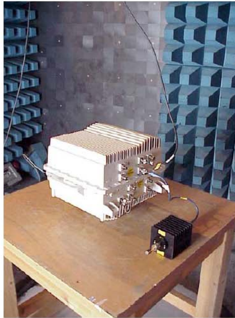
Photo 3. Test setup in anechoic chamber.
