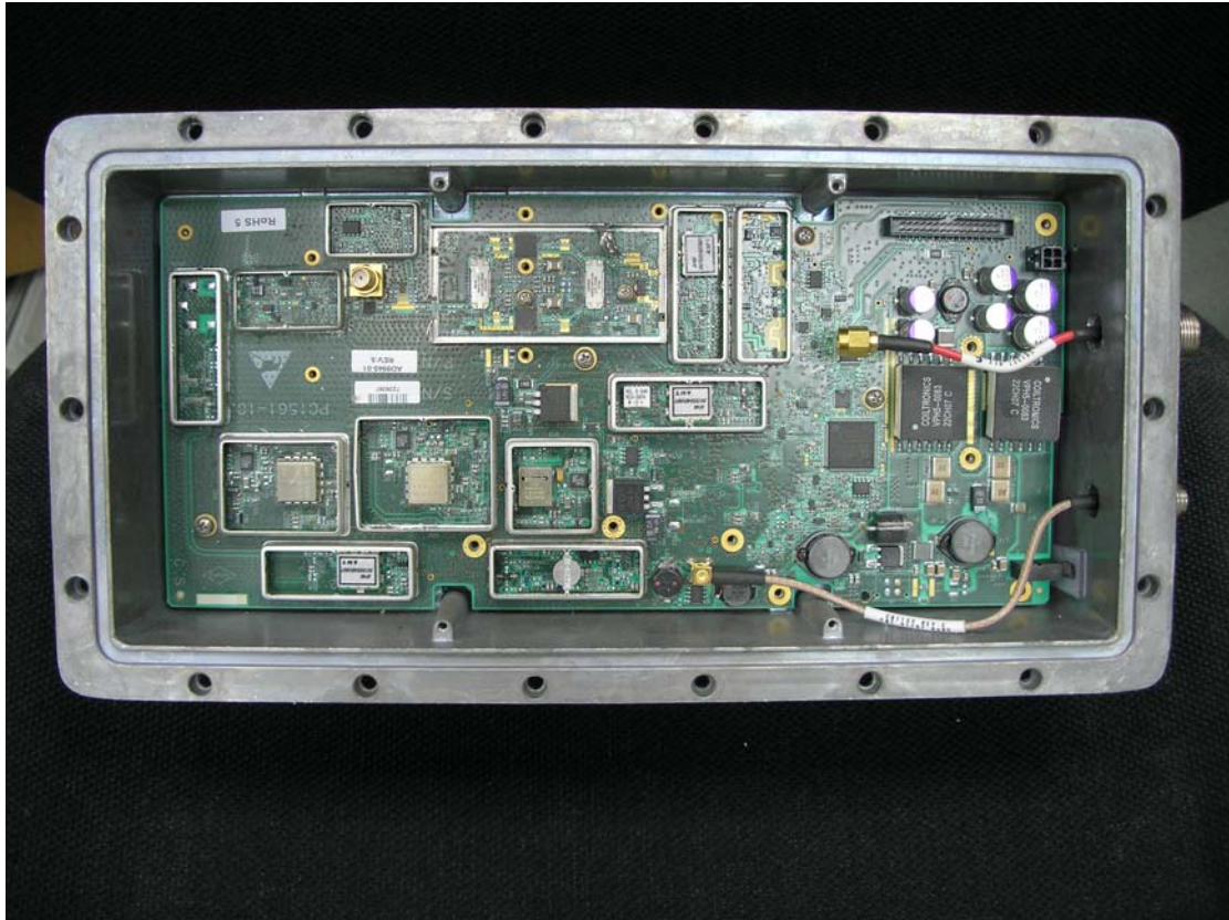
Photo3. ODU PCB components side view
