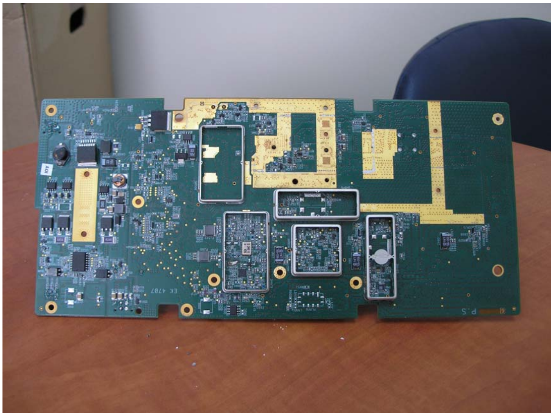
Photo4 . ODU, PCB print side
