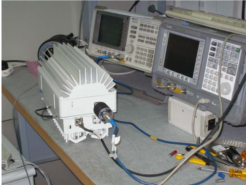
Antenna Port Tests Set Up
