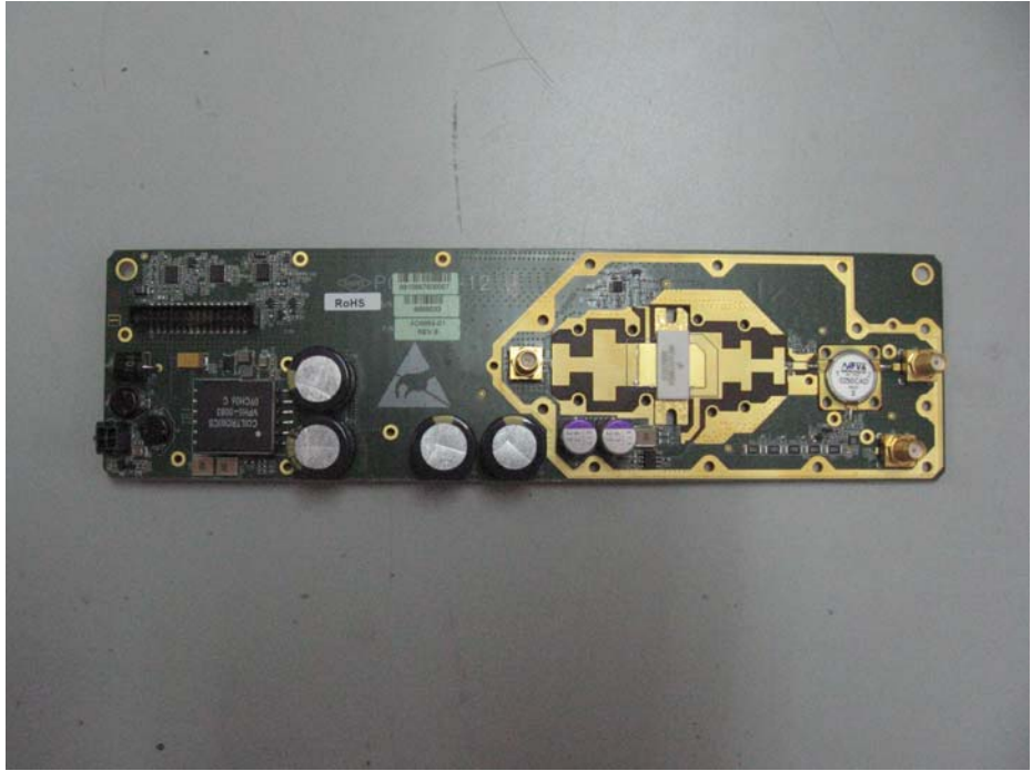
Power Amplifier PCB CS
