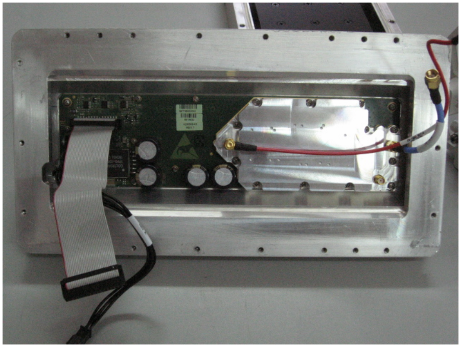
Power Amplifier In Case With Open Cover
