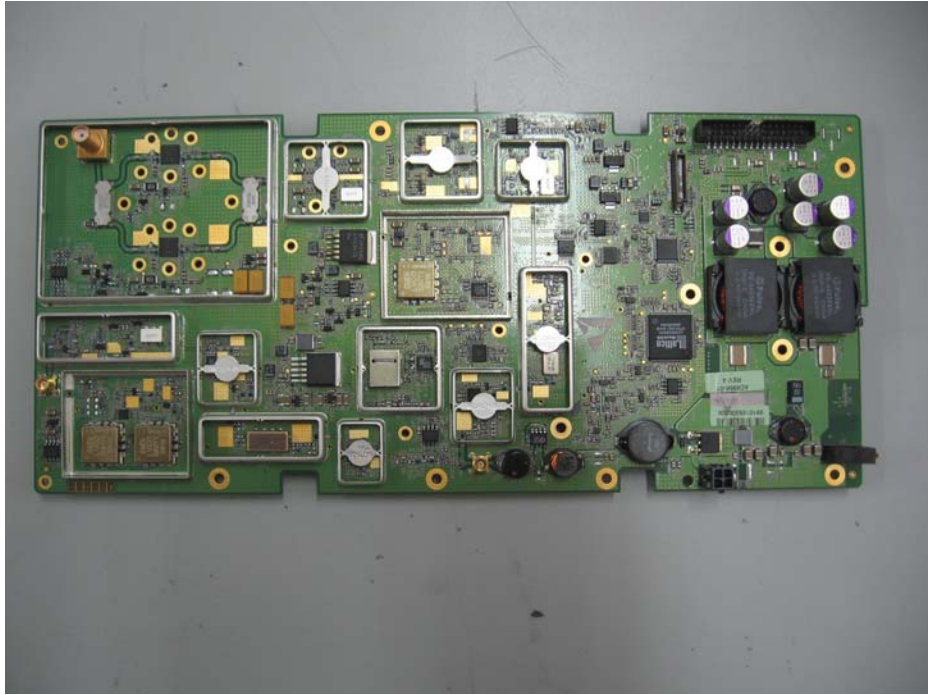
Pasic Unit PCB CS Without Cover
