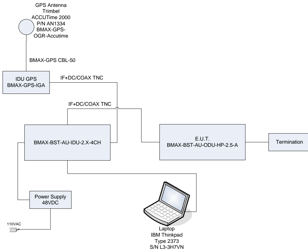
Figure 3. Tests Set-up
