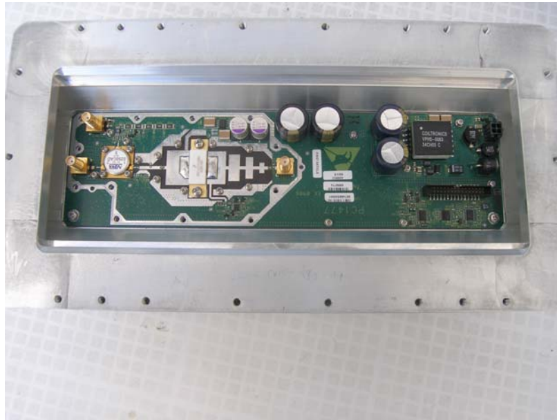
Photo 3 Power amplifiers PCB, open cover CS
