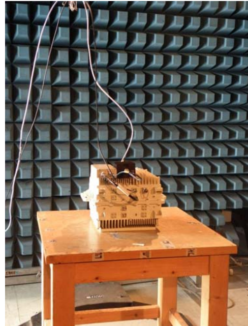
Measurement of radiated emission
