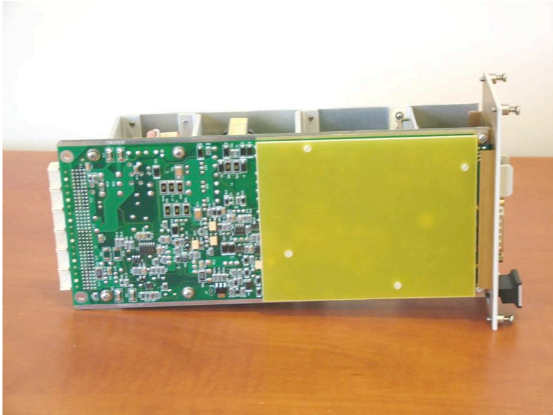
Base station indoor , DC Power supply Print side
