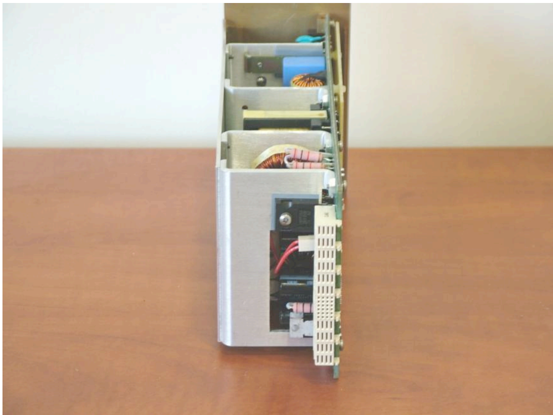
Base station indoor , DC Power supply connector side
