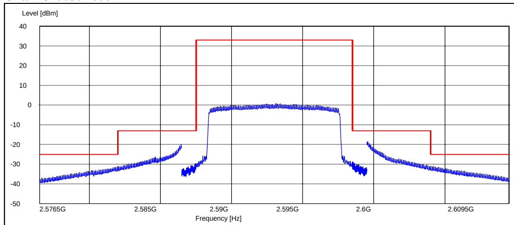
Channel 368 / 2593MHz
