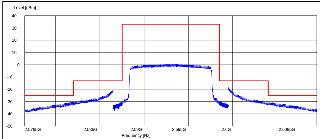
Channel 368 / 2593MHz
