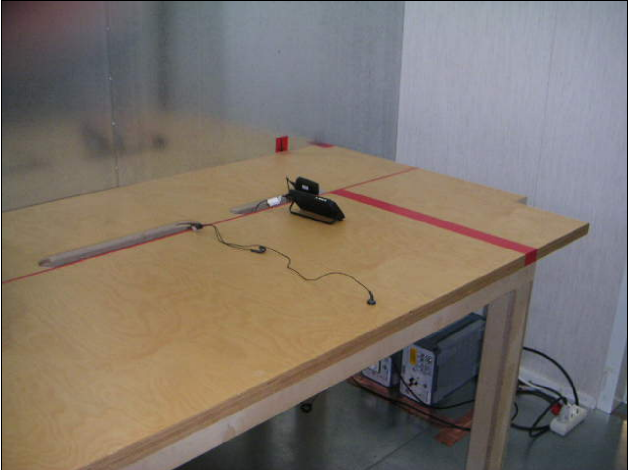
Picture 2 AC powerline conducted emission measurement Bluetooth TX
