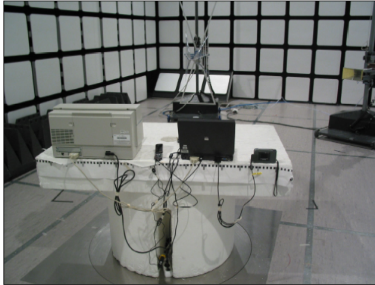
Picture 5 Radiated emission measurement setup
