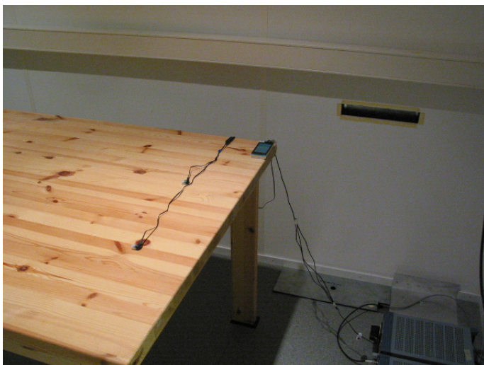
Picture 3 AC powerline conducted emission measurement 15C
