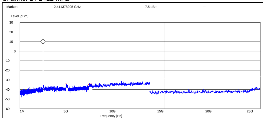
Channel 1 / 2412 MHz
