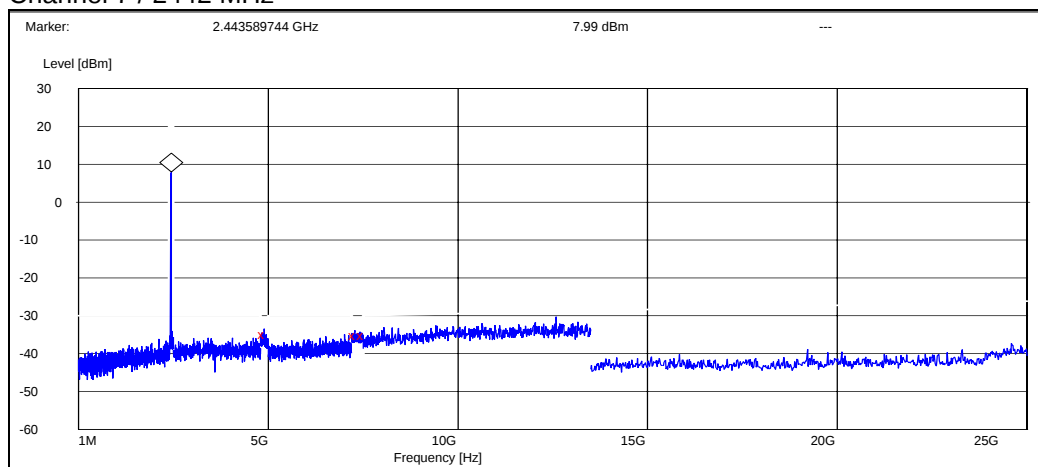
Channel 7 / 2442 MHz
