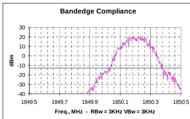
Picture 6. Lower bandedge, channel 512 GSM
