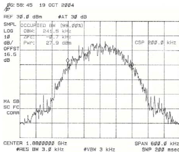
Picture 5. 99% occupied bandwidth EGPRS, channel 661
