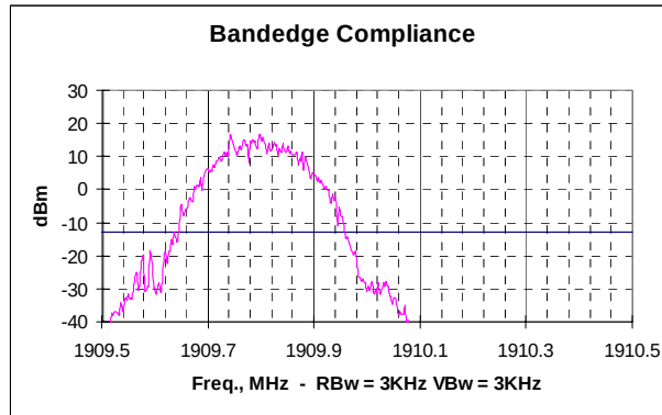
Picture 7. Upper bandedge, channel 810 EGPRS
