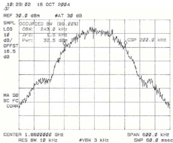
Picture 4. 99% occupied bandwidth GSM, channel 661
