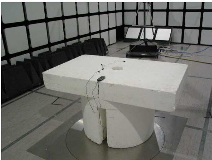
Picture 2 Radiated emission measurement GSM RX + FM radio on
