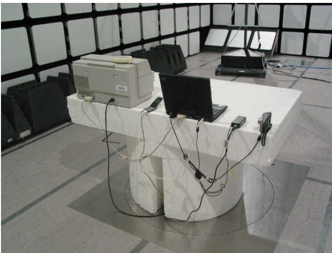
Picture 2 Radiated emission measurement GSM RX/WLAN TX + Computer peripherals
