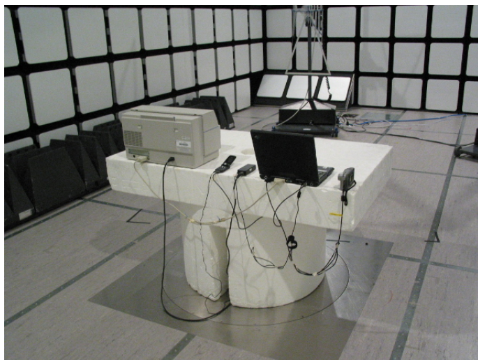
Picture 2 Radiated emission measurement WLAN TX + Computer peripherals
