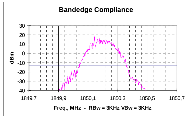
Picture 8. Lower bandedge, EGPRS channel 512
