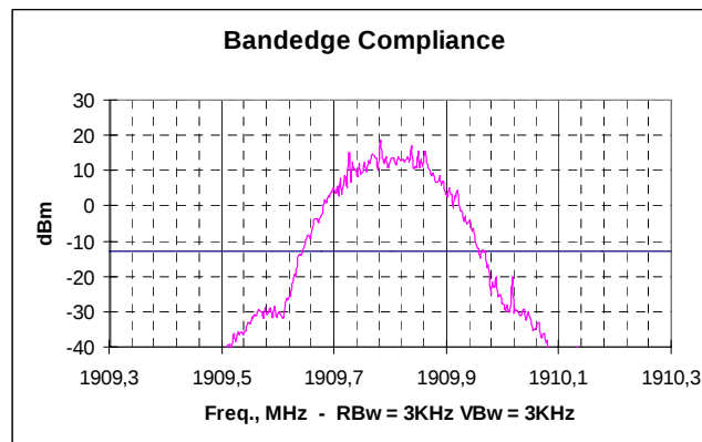
Picture 9. Upper bandedge, EGPRS channel 810
