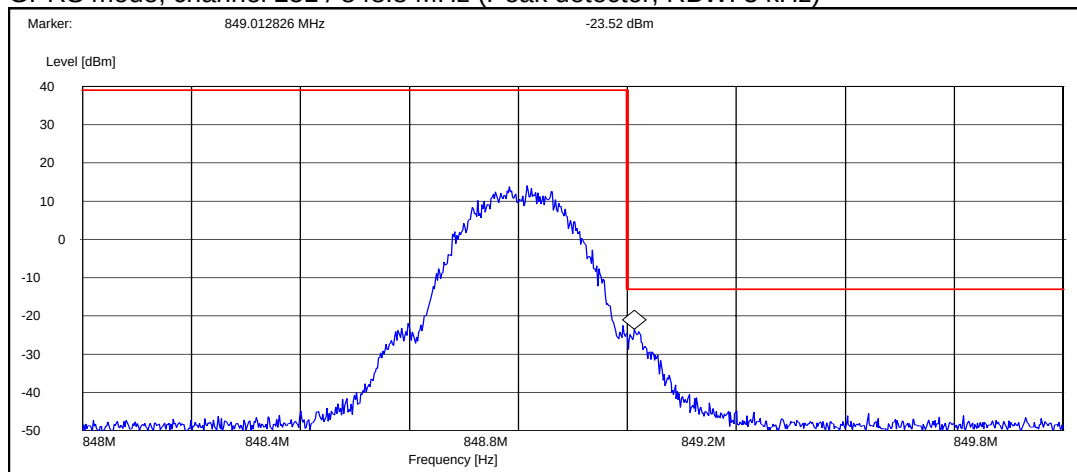
GPRS mode, channel 251 / 848.8 MHz (Peak detector, RBW: 3 kHz)
